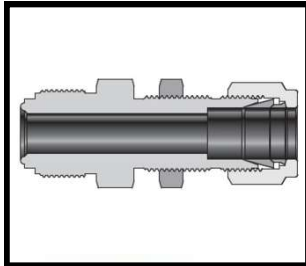
BTF-BODY TO BULKHEAD TUBE FITTING
